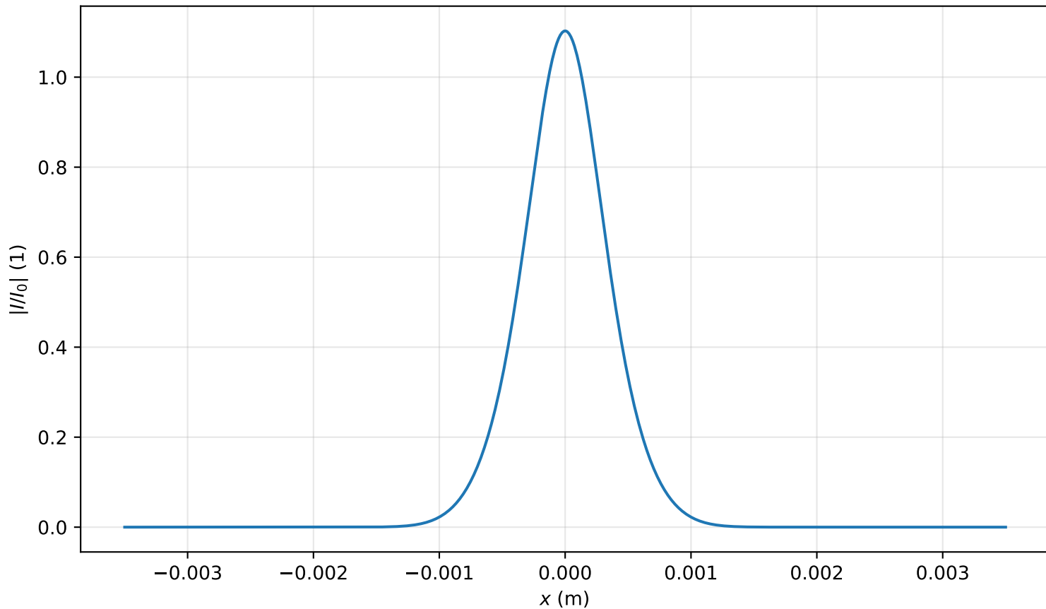
Intensity profile I(x, y = 0, z = 0.716m)/I_0 , P_{in}=0.6P_{cr} , artificial time
